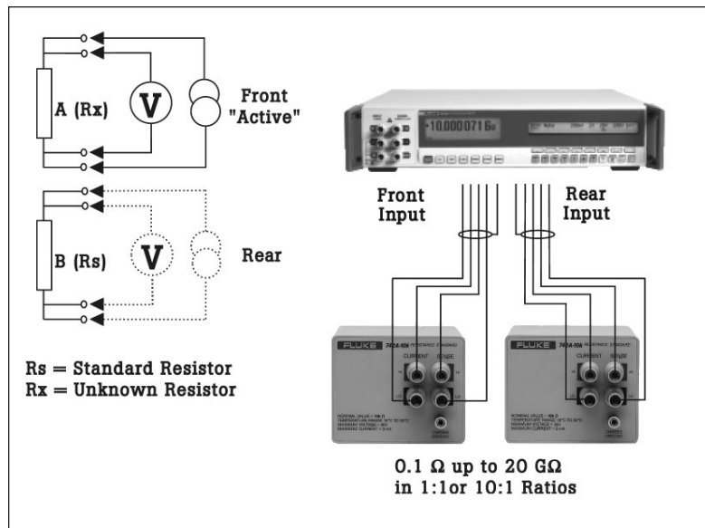
Fig. 9 Resistance ratio.
