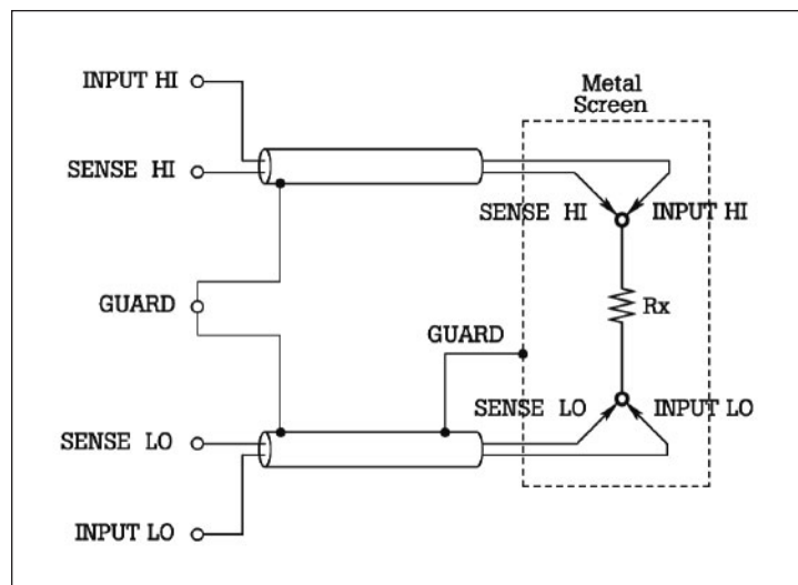
Fig. 7 Ohms guard connections.
